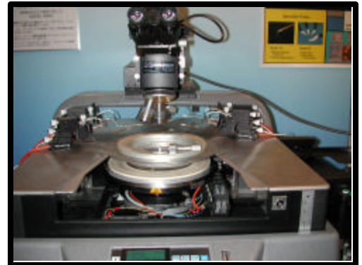
220 mm multi-site card on 9920 (300mm) probe station
