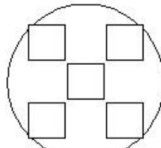
Five 46 mm Tiles over 200 mm wafer
